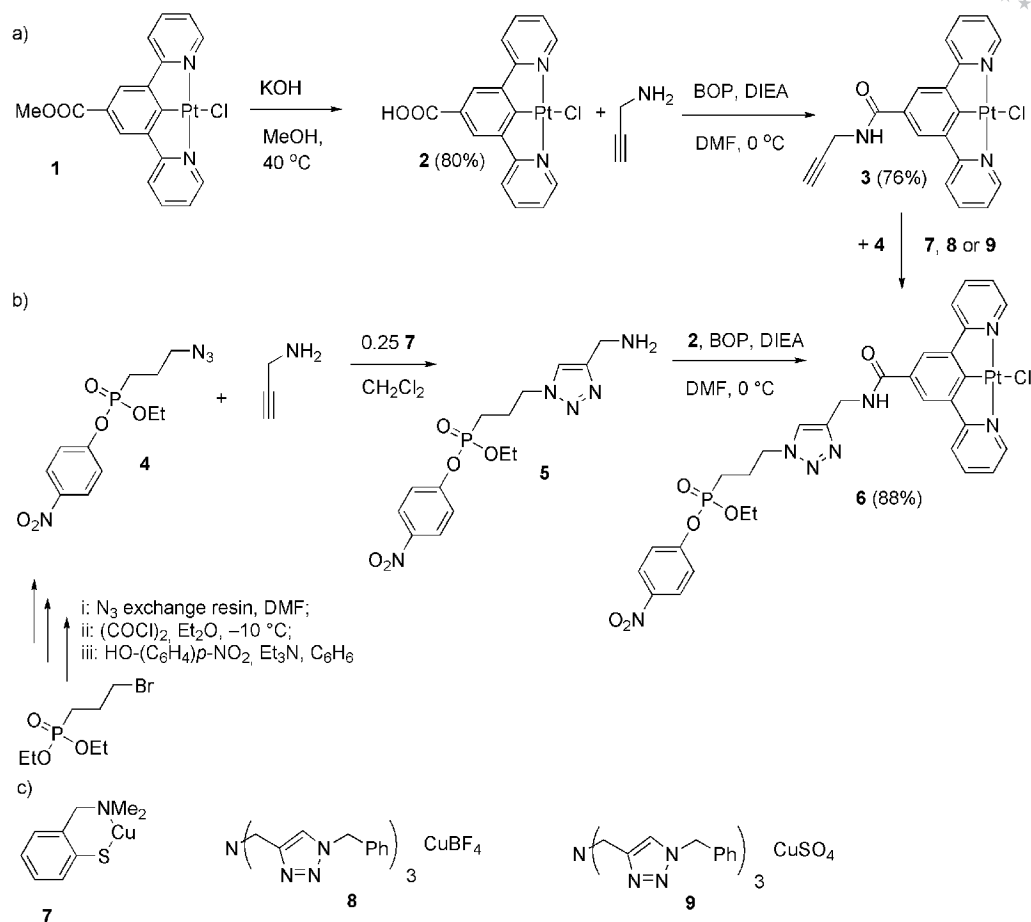
Scheme 1. Explored routes (a) and (b) towards the synthesis of the luminescent pincer platinum phosphonate inhibitor 6 ; the different tested click catalysts are shown under (c).
