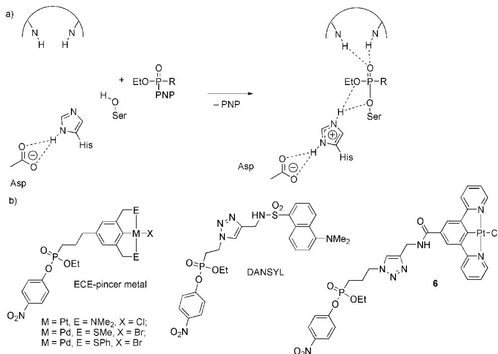
Figure 1. (a) General inhibition reaction of serine hydrolases with phosphonates (PNP = p -nitrophenolate anion). (b) Structures of organometallic ECE-pincer-metal phosphonates (left), [20,21] of an organic luminescent dansyl phosphonate inhibitor (middle) [22] and of the organometallic luminescent target inhibitor 6 (right).
