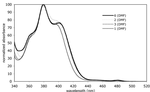
Figure 2. Normalized absorption spectra of NCN–platinum complexes 1–3 and inhibitor 6 in DMF.
