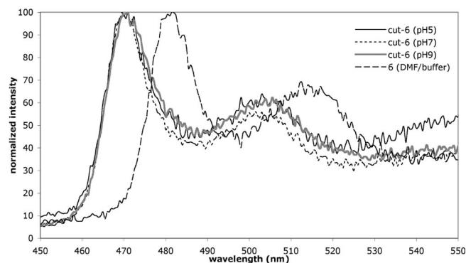
Figure 6. Normalized luminescence spectra of cut-6 at pH 5, 7 and 9 in Tris/Triton buffer; for comparison, the spectrum of inhibitor 6 in DMF/buffer (1:1 v/v, buffer: Tris/Triton, pH 8.0) has been included.
