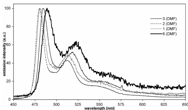
Figure 3. Normalized emission spectra of NCN–platinum complexes 1–3 and inhibitor 6 in DMF.
